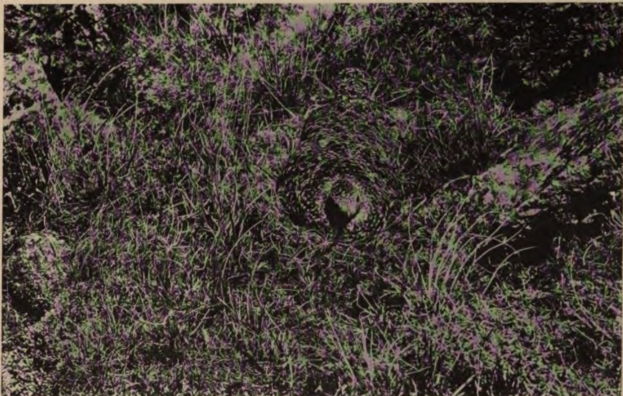
FIG. 40. Rocky Mountain White-tailed Ptarmigan on her nest. Near-ground-picturing pattern, of the grass-type 'based, of course, on full obliterative shading.) [See p. 47, Chap. VII.] Photographed from life by Evan Lewis.
